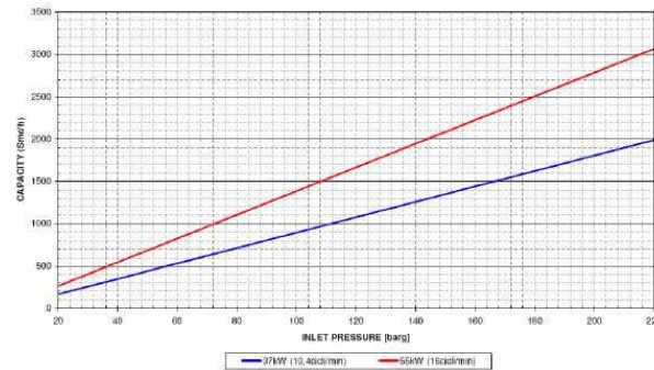
BOOSTER B37-55 PERFORMANCES
